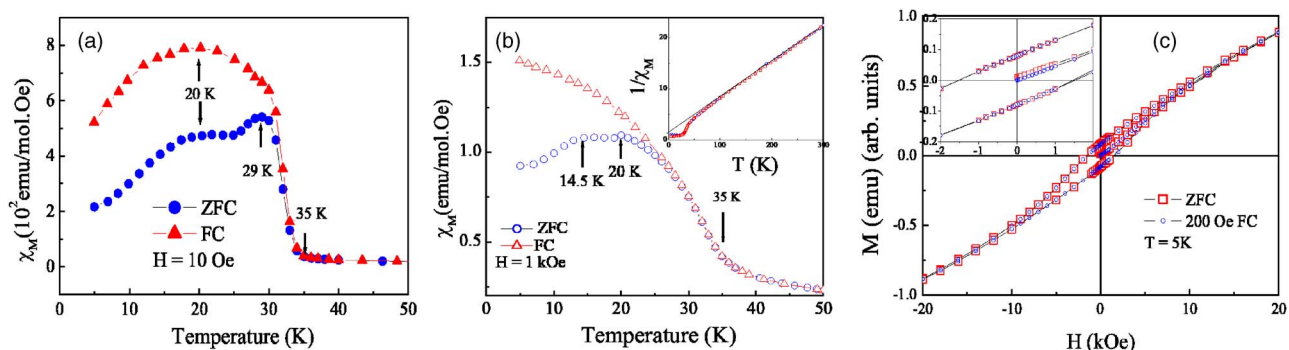
FIG. 3. Temperature variation of \chi_M for the SrHo 2 116, x=0 crystals for (a) H=10 Oe and (b) 1 kOe (inset \chi_M^{-1} vs T ). (c) M - H curves recorded at 5 K in ZFC and 200 Oe FC condition; inset gives an enlargement of the low field region.
