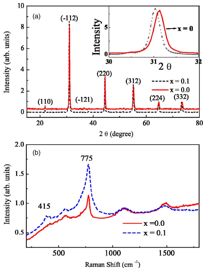
FIG. 2. (a) XRD patterns of the SrHo 2 116 crystals at x=0 (solid line) and x=0.1 (dashed line) and (b) Raman spectra of x=0.0 (solid line) and x=0.1 (dashed line) crystals.
