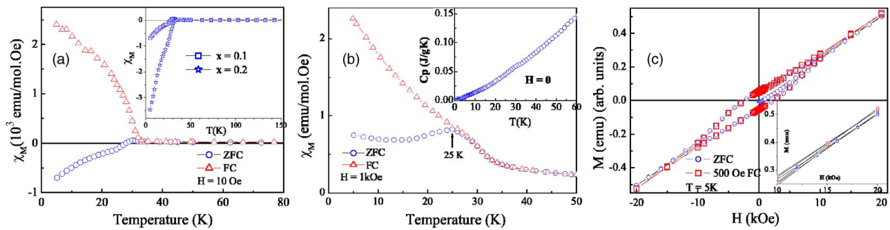
FIG. 4. Temperature variation of \chi_M for the SrHo2116, x=0.1 crystals recorded at H=10 Oe (a) and H=1 kOe (b), inset giving the C_p vs T variation at H=0 . (c) ZFC (circle) and 500 Oe FC (squares) M-H curves of x=0.2 crystal recorded at 5 K; inset gives an enlargement of a section in high field region.
