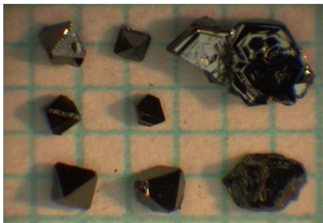
FIG. 1. Optical micrograph of SrHo2116 crystals grown at 1200 °C.
